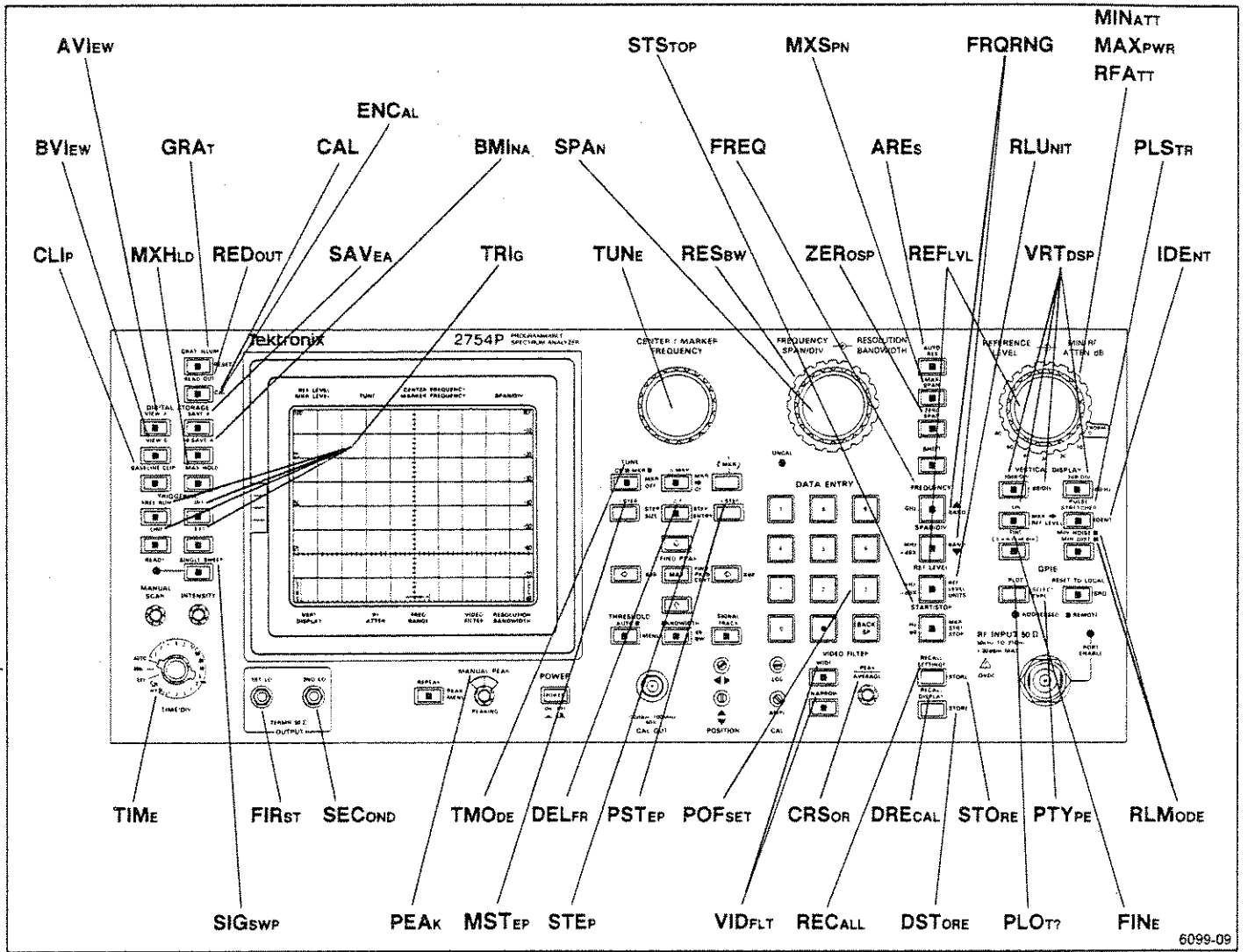
Figure B-1. TEKTRONIX 2754P Spectrum Analyzer
